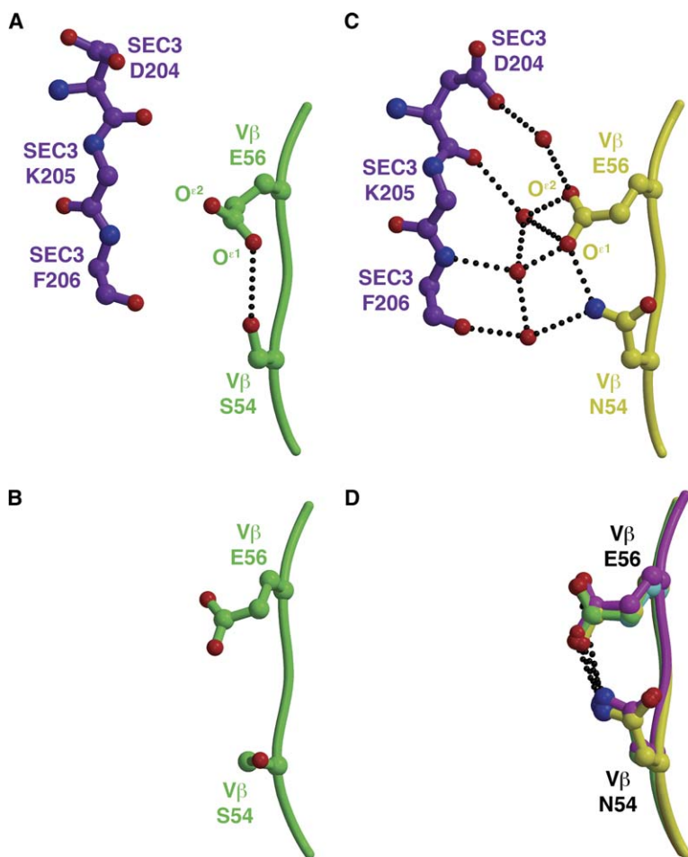
Figure 4. The S54N Vβ Mutation Modulates the Conformation of the Invariant Residue Glu56 to Facilitate an Extensive Water-Mediated Hydrogen Bonding Network with SEC3 (A) An intramolecular hydrogen bonding interaction between S54 Vβ and E56 Vβ prevents interactions and intermolecular contacts with SEC3. (B) The analogous region of the CDR2 loop of wild-type apo Vβ. (C) The mutation S54N Vβ extends both N54 Vβ and E56 Vβ side chains toward SEC3, resulting in the recruitment of numerous ordered water molecules to the molecular interface. (D) The relative conformations of the N54 Vβ and E56 Vβ side chains are ordered prior to binding SEC3, as seen in all apo Vβ variants containing the A52V Vβ mutation for which we have determined crystal structure. Hydrogen bonds are shown as black, dotted lines.
