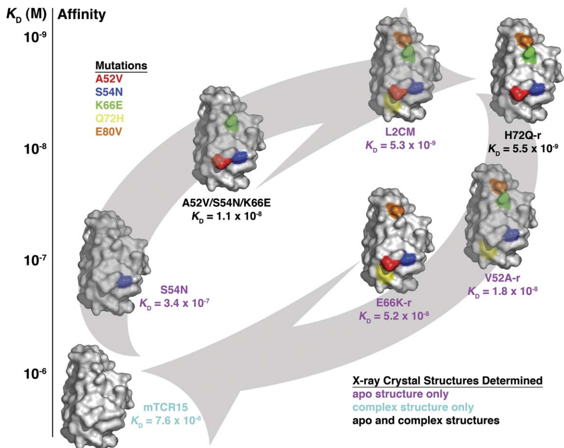
Figure 2. Overview of the Crystallographic Analysis of the Affinity Maturation and Reversion Pathways in the V \beta -SEC3 Interaction V \beta variants are shown as molecular surface representations; only residues that are in their mutated stated highlighted by the following colors: A52V, blue; S54N, red; K66E, green; Q72H, yellow; and E80V, orange. Arrows indicate the affinity maturation pathway (from wild-type toward L2CM, bottom left to top right) and the affinity reversion pathway (from L2CM to wild-type, from top right to bottom left). V \beta variants are plotted according to their relative affinities for SEC3 (vertical axis) and are placed on the appropriate affinity modulation pathway. Labels of each V \beta variant are color coded to reveal which crystal structures were determined as follows: apo V \beta crystal structure only, magenta; V \beta -SEC3 complex crystal structure only, cyan; both apo V \beta and V \beta -SEC3 complex crystal structures, black. In our naming convention of this affinity maturation pathway, wild-type V \beta and L2CM (highest affinity/fully matured V \beta variant) define the energetic start and end points of the pathway, respectively. Intermediate V \beta variants are described by the particular mutation or combination of mutations found in the variant, with a -r label distinguishing reversion mutations from their maturation counterparts.
