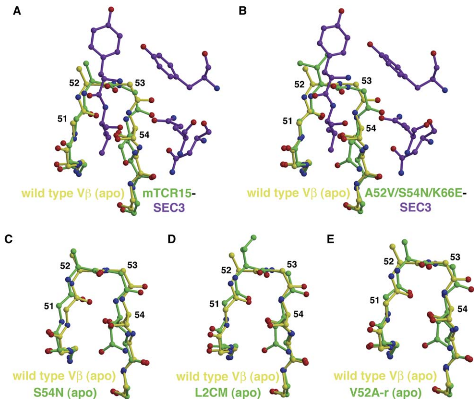
Figure 7. Flexibility of the Vβ CDR2 Loop
