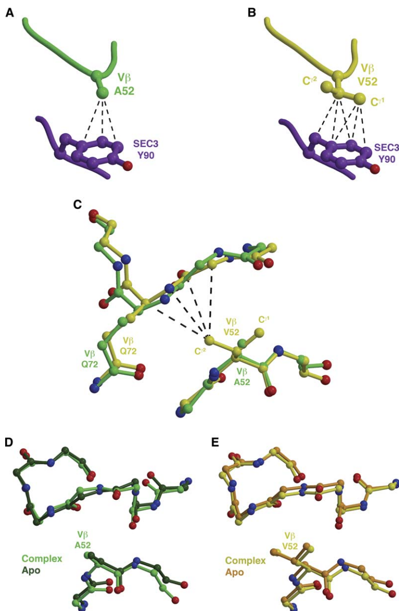
Figure 3. Multiple Structural Consequences of the A52V Vβ Mutation
