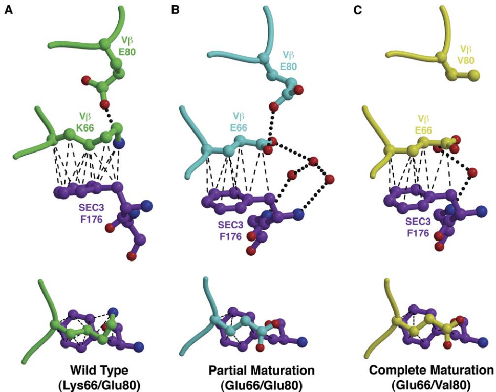
Figure 5. Molecular Interplay between Variant Residues at Positions 66 Vβ and 80 Vβ
