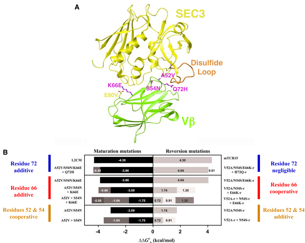
Figure 1. Relative Positions of V \beta Variant Residues and Energetic Consequences of Their Variation
