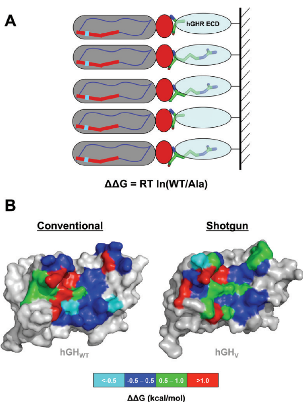
Figure 5. Shotgun alanine mutagenesis of a high-affinity variant of human growth hormone (hGH V ). (A) Schematic of shotgun alanine mutagenesis. For each position of interest, arginine (in this case) is mutated to alanine. Both are incubated with human growth hormone receptor, and the ratio of the wild type (WT) to alanine is calculated from sequencing data. This is related to the change in the Gibbs free energy upon mutation. (B) Surface residues of hGH WT (left) and hGH V (right) that were scanned by alanine mutagenesis and shotgun alanine mutagenesis, respectively (Protein Data Bank entries 3hrh and 1kf9, respectively). Residues are colored according to \Delta\Delta G_{\text{Ala-X}} : red for >1.0 kcal/mol, green for 0.5-1.0 kcal/mol, blue for 0.5 to -0.5 kcal/mol, cyan for less than -0.5 kcal/mol, and gray for untested.
