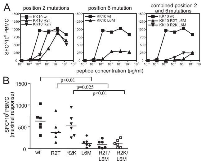
Figure 1. Consistent lack of recognition of the KK10 L6M variant by KK10-specific CD8 + T cells during primary HIV-1 infection.
